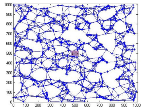
Fig 1. Kneigh Topology( k=9 )
