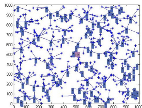
Fig. 2 NCTC topology
